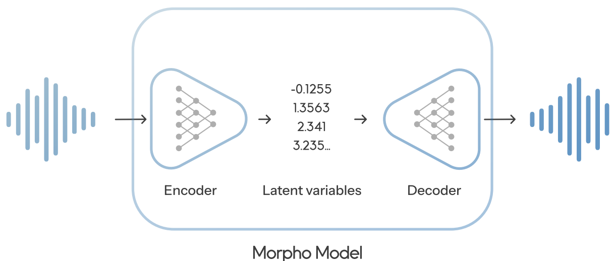
A diagram of neutone morpho algorithm
